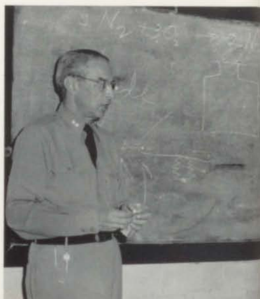
CAPT. JOHN A. BRADFORD A.B., Randolph Macon Science, Mathematics 1 Year at M.M.I.
